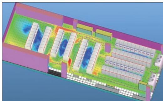
▲An example of iDC thermal airflow analysis Analysis software: TileFlow (Innovative Research Company)
